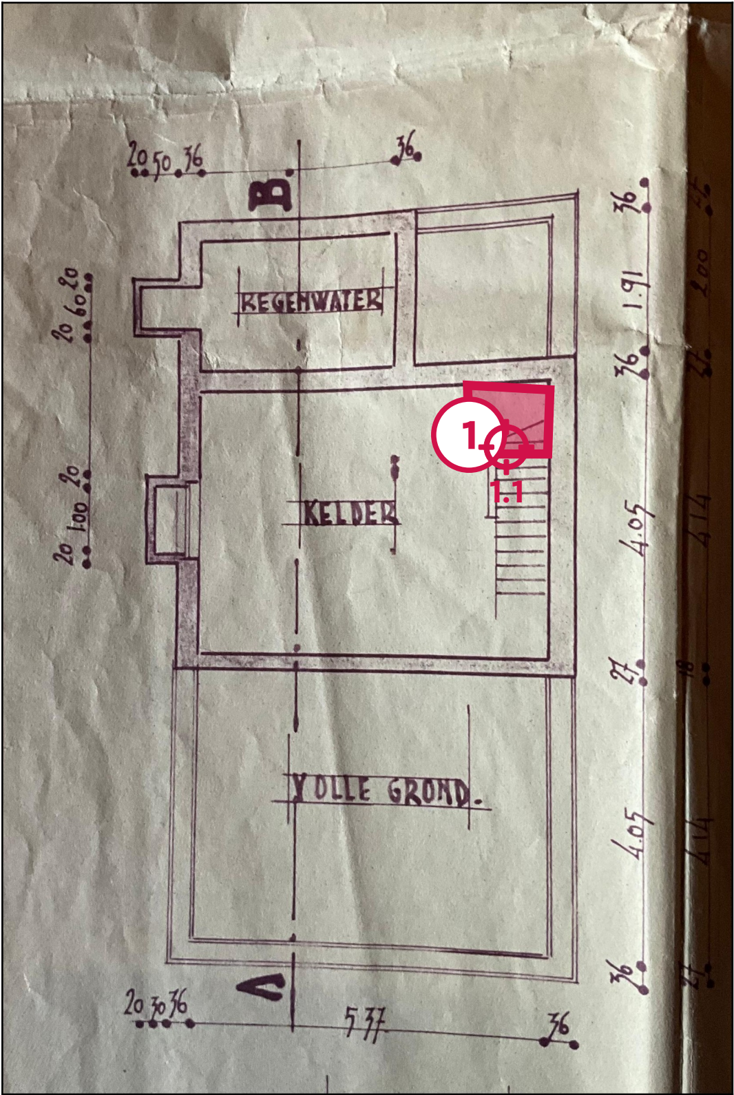
Legende van plan 1.8: kelder
