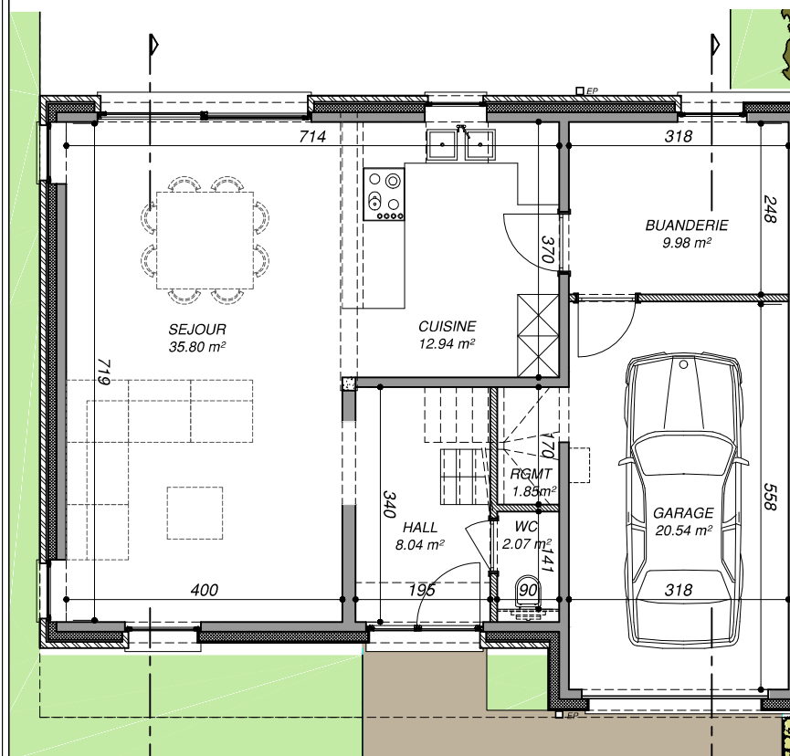
Plan REZ
