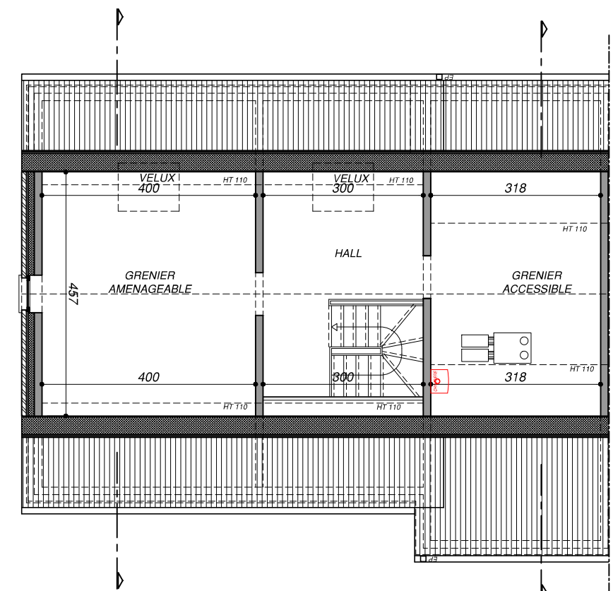
Plan COMBLES
