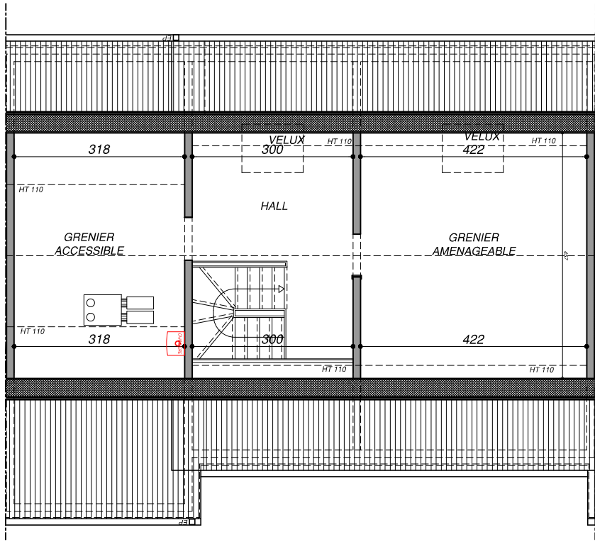
Plan COMBLES
