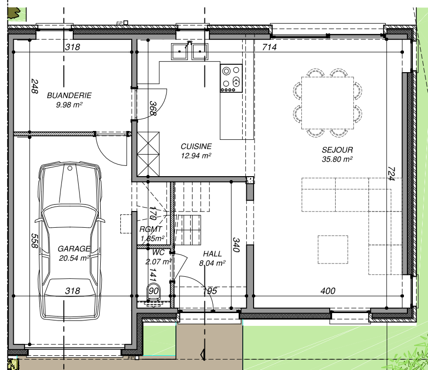
Plan REZ
