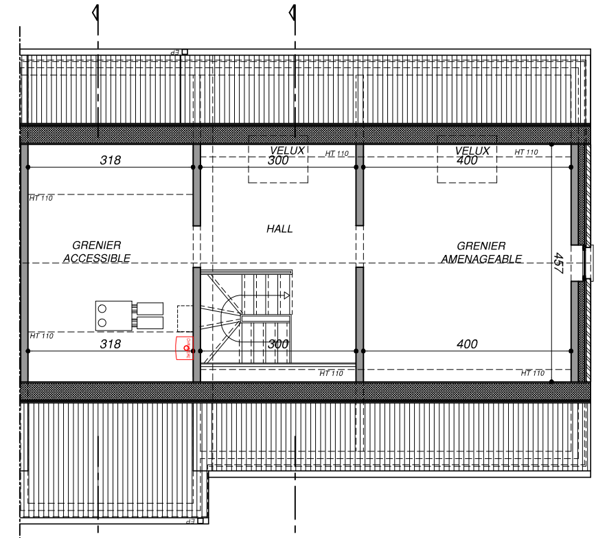
Plan COMBLES
