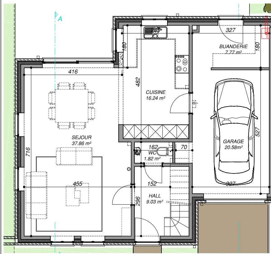
Plan REZ
