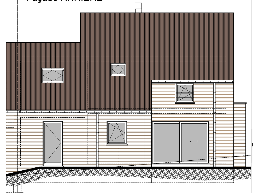
Façade ARRIERE
