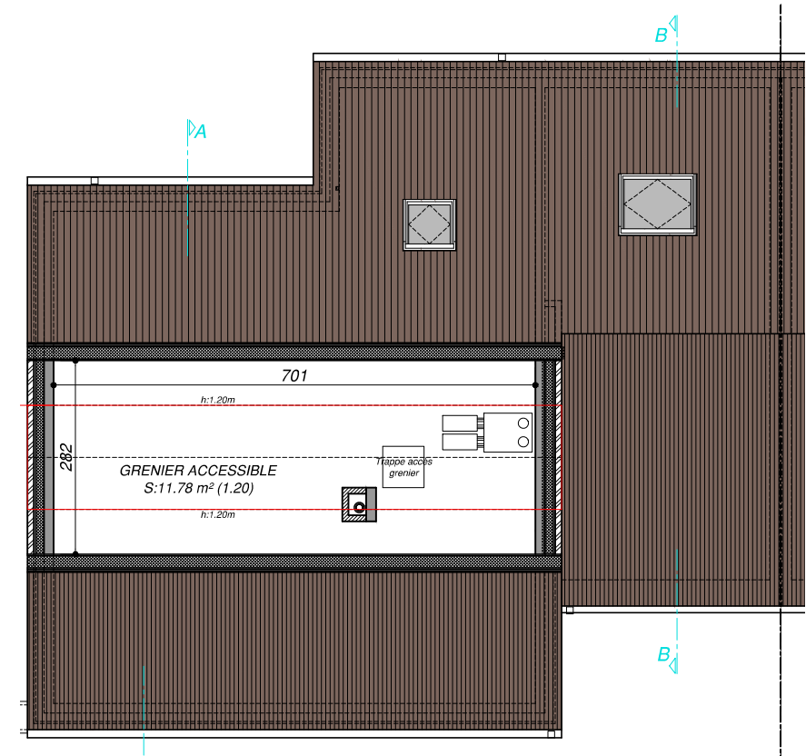
Plan COMBLES
