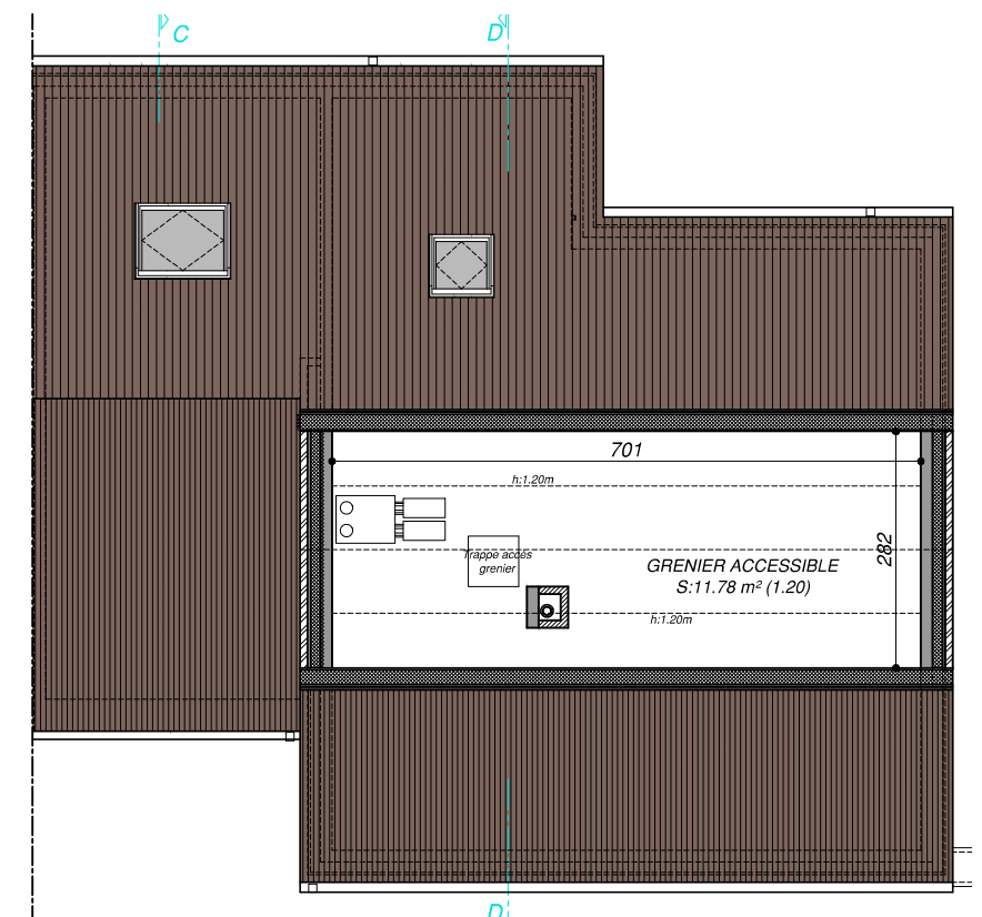
Plan COMBLES
