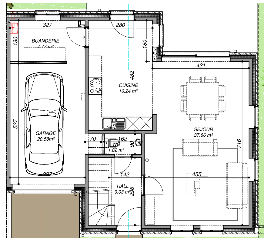
Plan REZ
