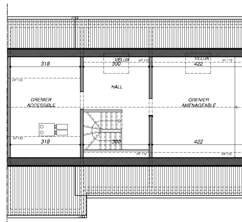
Plan COMBLES
