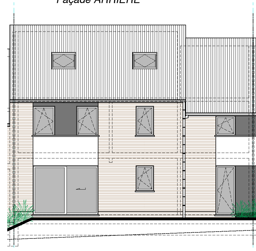
Façade ARRIERE
