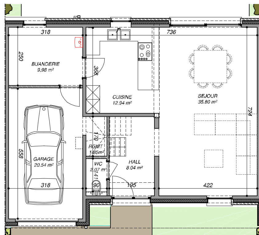
Plan REZ
