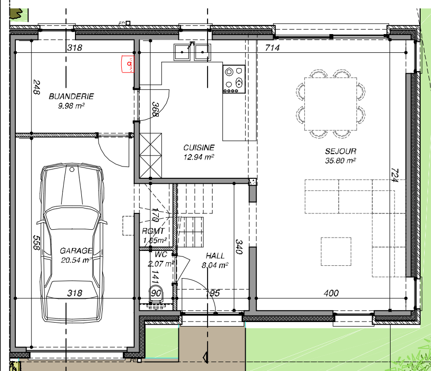
Plan REZ
