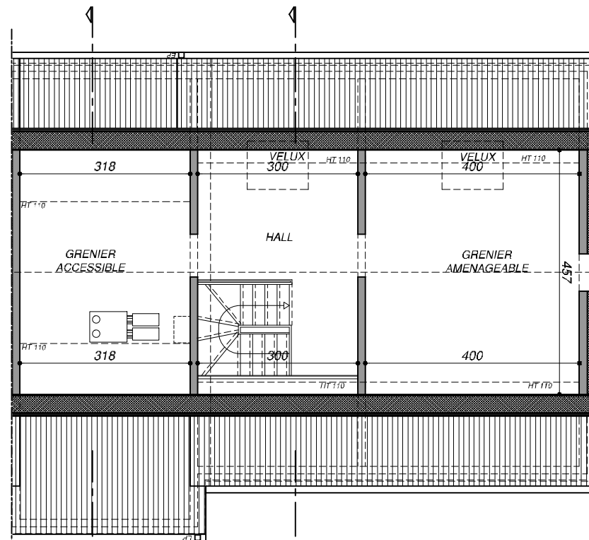
Plan COMBLES
