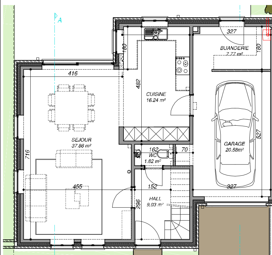
Plan REZ
