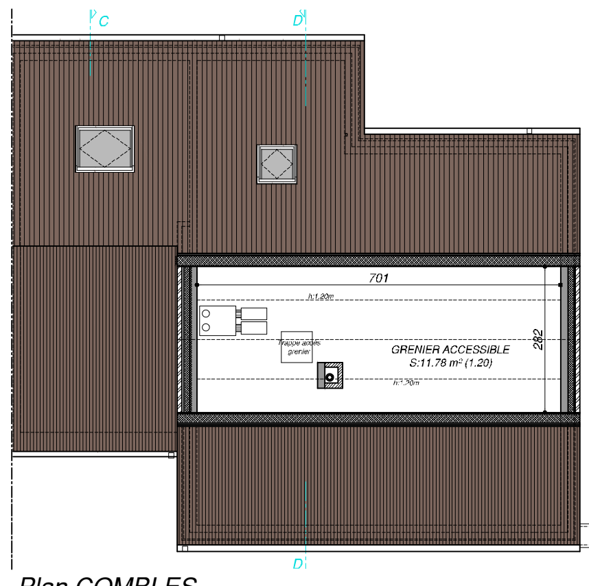
Plan COMBLES
