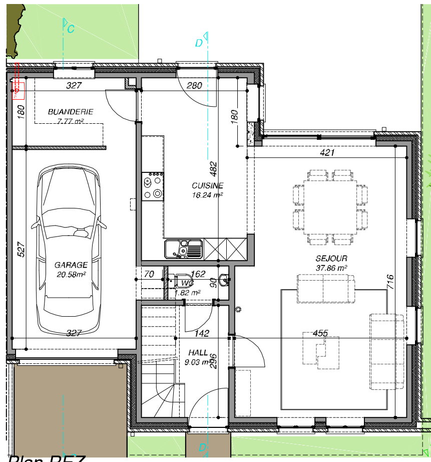
Plan REZ
