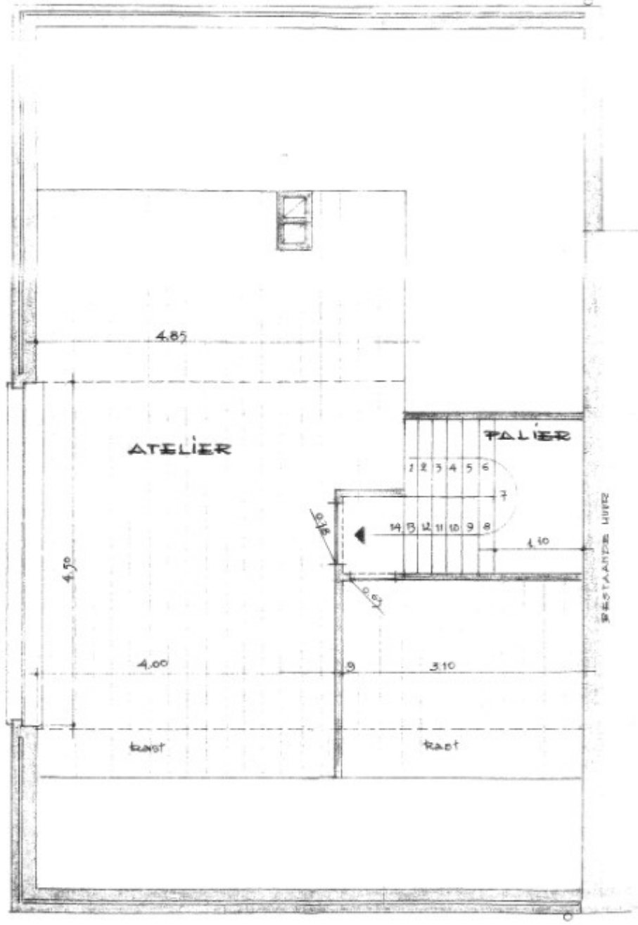
ZOLDERPLAN
