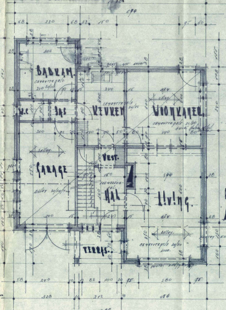
BEGANE GOND
